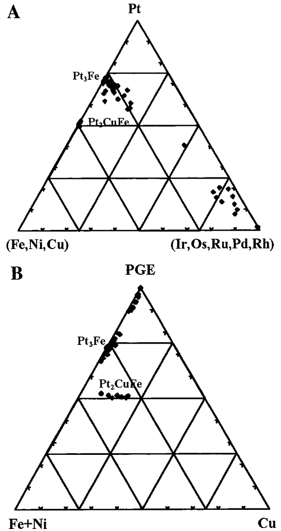
FIG. 3. Composition of Pt-Fe, Pt-Fe-Cu and Os-Ir alloys from the Goodnews Bay placer. A. Plots of alloy compositions on a (Fe,Ni,Cu) - Pt - (Ir,Os,Ru,Pd,Rh) diagram, showing trend of differentiation between isoferroplatinum and iridium. B. Plots of composition of primary minerals without Cu and a series of secondary tulameenite compositions in terms of (Fe+Ni) - PGE - Cu.
