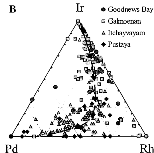
FIG. 7. Ratio of minor elements contents in isoferroplatinum from the Goodnews Bay placer in comparison with some other Alaskan-type occurrences (A), and the Kamchatka district (B). Arrows indicate the trend of the change of Pt–Fe alloy composition with decreasing temperature of ore formation.
