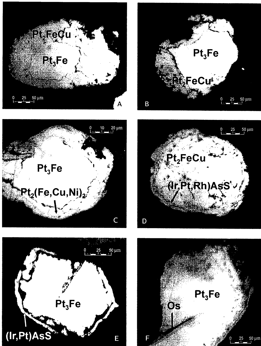
FIG. 2. Scanning-electron microscope images, showing relationships among PGM. A,B,C. Grains of isoferroplatinum surrounded by a tulameenite rim. D. Tulameenite with a rim of secondary irarsite. E. Isoferroplatinum grains surrounded by irarsite. F. Inclusion of osmium in isoferroplatinum, which is surrounded by irarsite.
